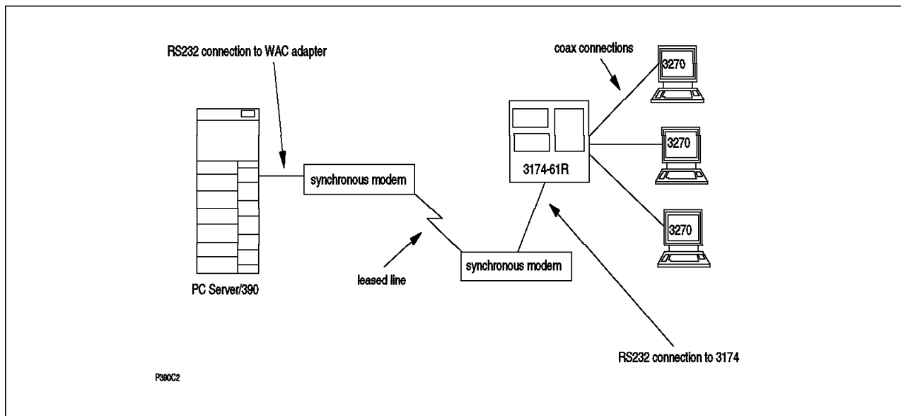
Figure 33. Trial SDLC Configuration. Note that synchronous modems are needed; typical PC modems are asynchronous and cannot be used for a basic SDLC connection. The 3174 is a widely-used control unit for 3270-family terminals. The 3174-61R is a remote version, used with up to eight terminals. Our unit was at microcode level C2.0.
