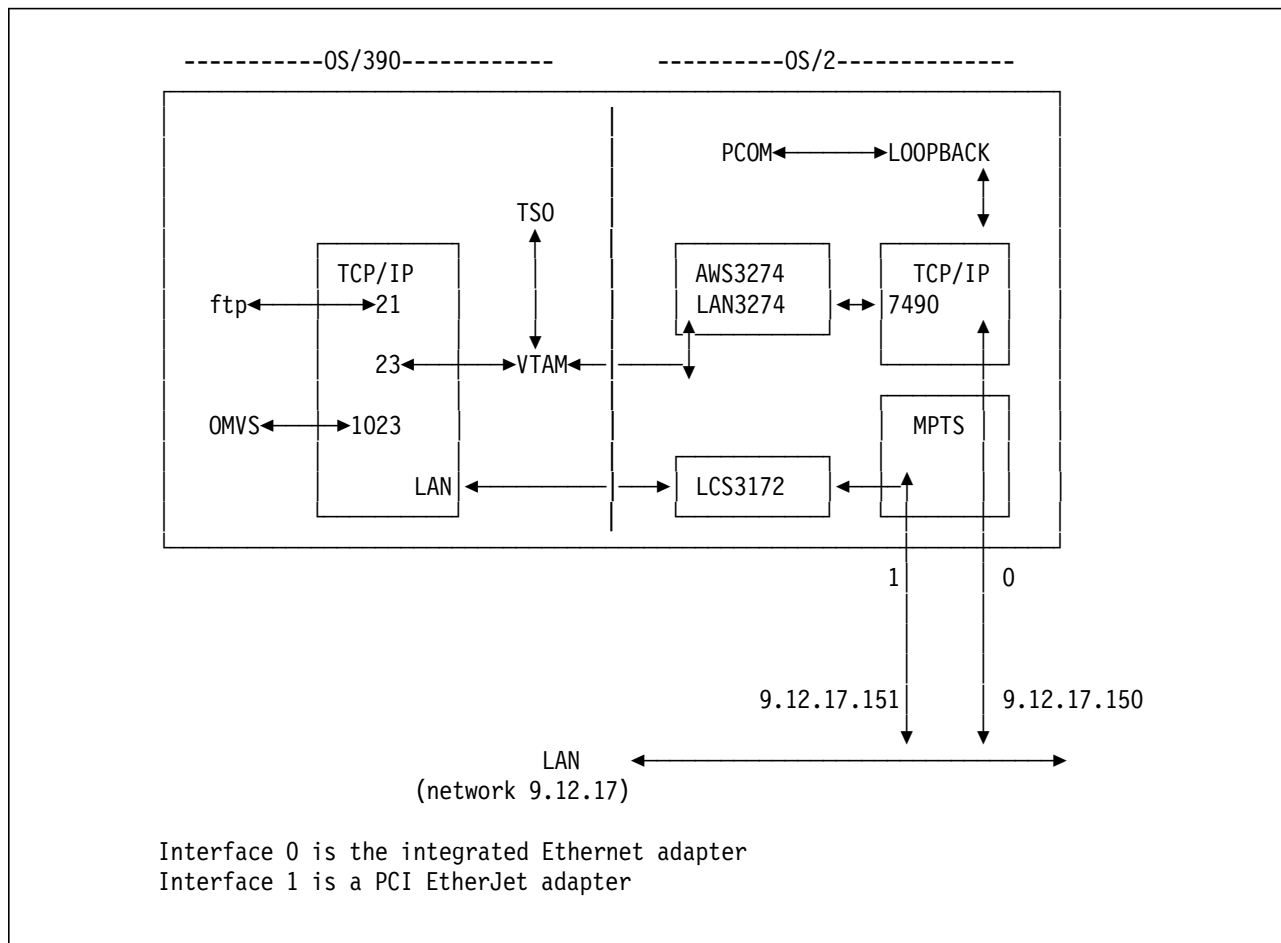
Figure 38. Goal for Basic P/390. This P/390 system has two LAN adapters. Adapter 0 is connected to OS/2 TCP/IP and the LAN3274 device manager. tn3270 sessions to port 7490 at 9.12.17.150 will appear to be local 3270 displays to OS/390. tn3270 sessions to port 23 at 9.12.17.151 will connect to OS/390 TCP/IP through the INTCLIEN server that connects them to VTAM. telnet sessions to port 1023 at address 9.12.17.151 will connect directly to OMVS. The PCOM sessions (on the OS/2 side) connect to OS/2 TCP/IP via the loopback address.
