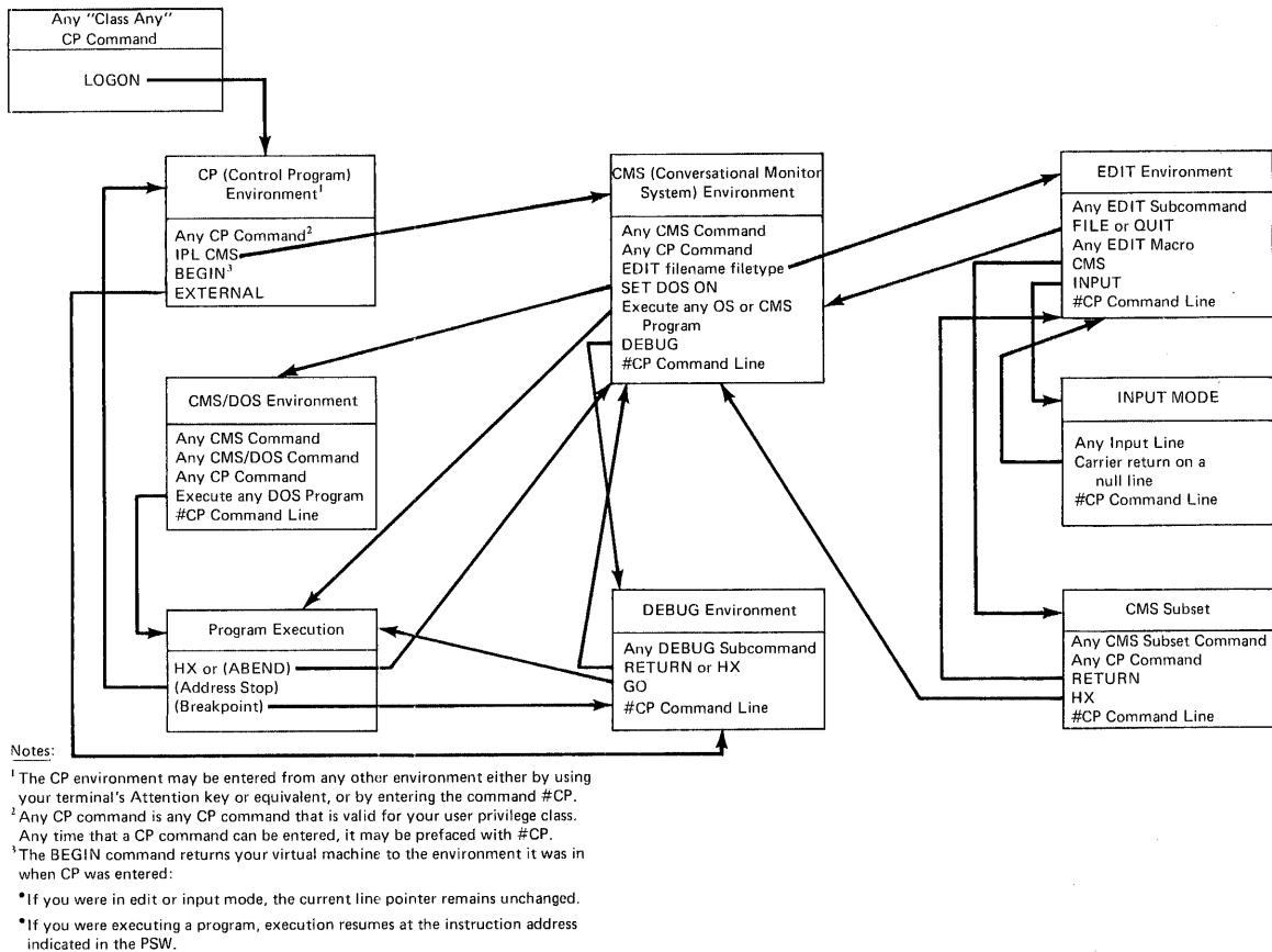
Figure 1. VM/370 Environments and Mode Switching
